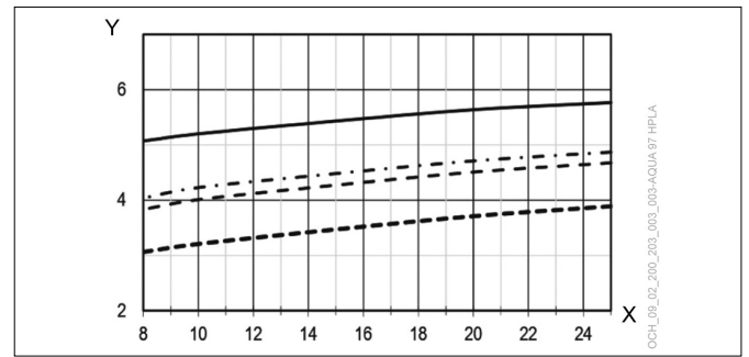
X Wassertemperatur [°C] Y COP
